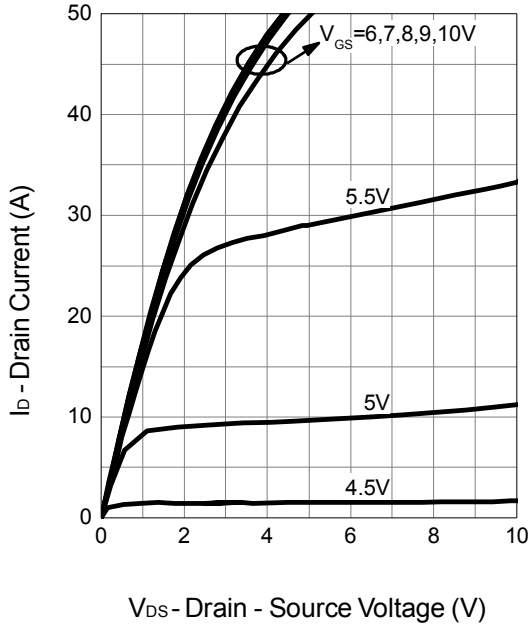
Output Characteristics
